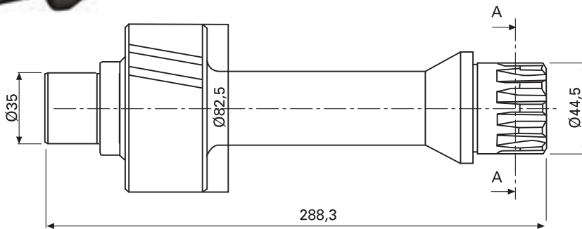
ZF 16 S 109 (13,53) KARDAN MİLİ ZF 16 S 109 (13,53) Cardan Shaft
