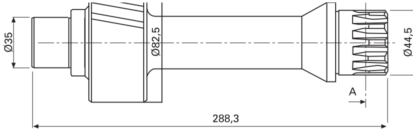
ZF 9 S 109 (12,92) KARDAN MİLİ ZF 9 S 109 (12,92) Cardan Shaft
